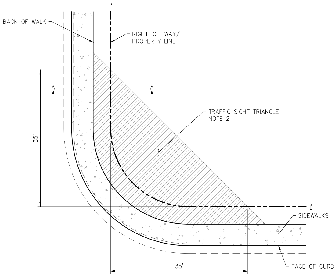
CORNER PLAN
